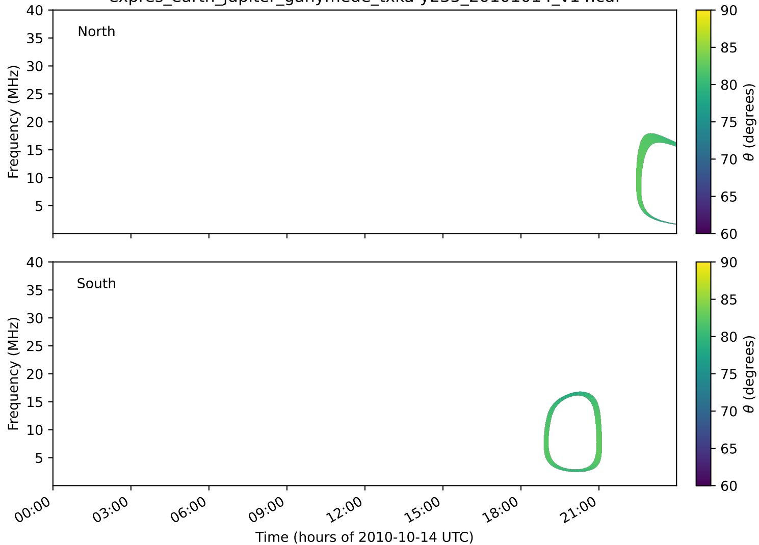
expres_earth_jupiter_ganymede_txka-y235_20101014_v14.cdf
