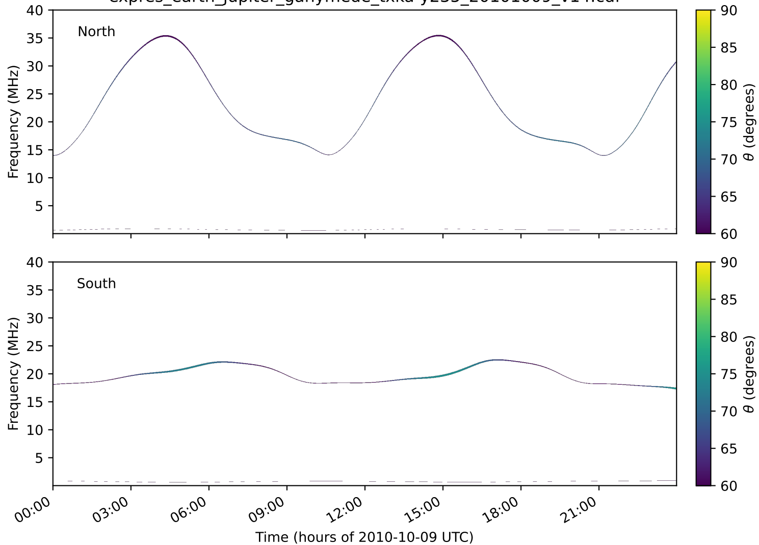
expres_earth_jupiter_ganymede_txka-y235_20101009_v14.cdf
