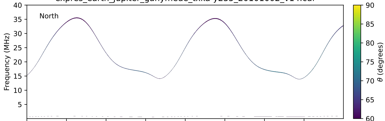
expres_earth_jupiter_ganymede_txka-y235_20101002_v14.cdf
