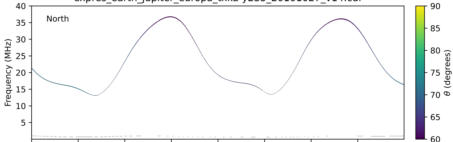
expres_earth_jupiter_europa_txka-y235_20101027_v14.cdf
