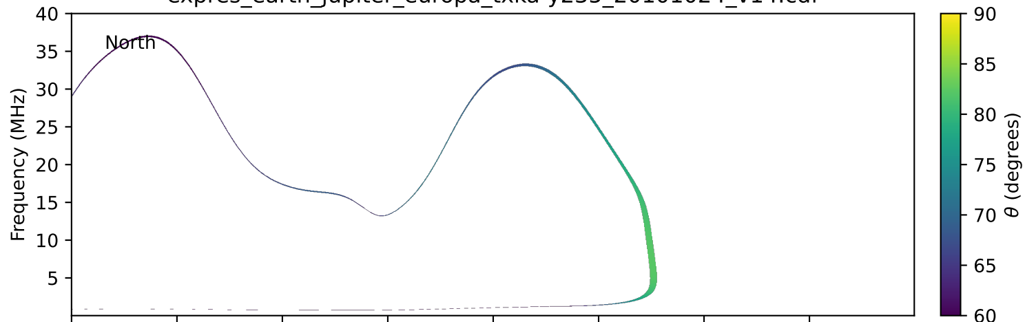
expres_earth_jupiter_europa_txka-y235_20101024_v14.cdf
