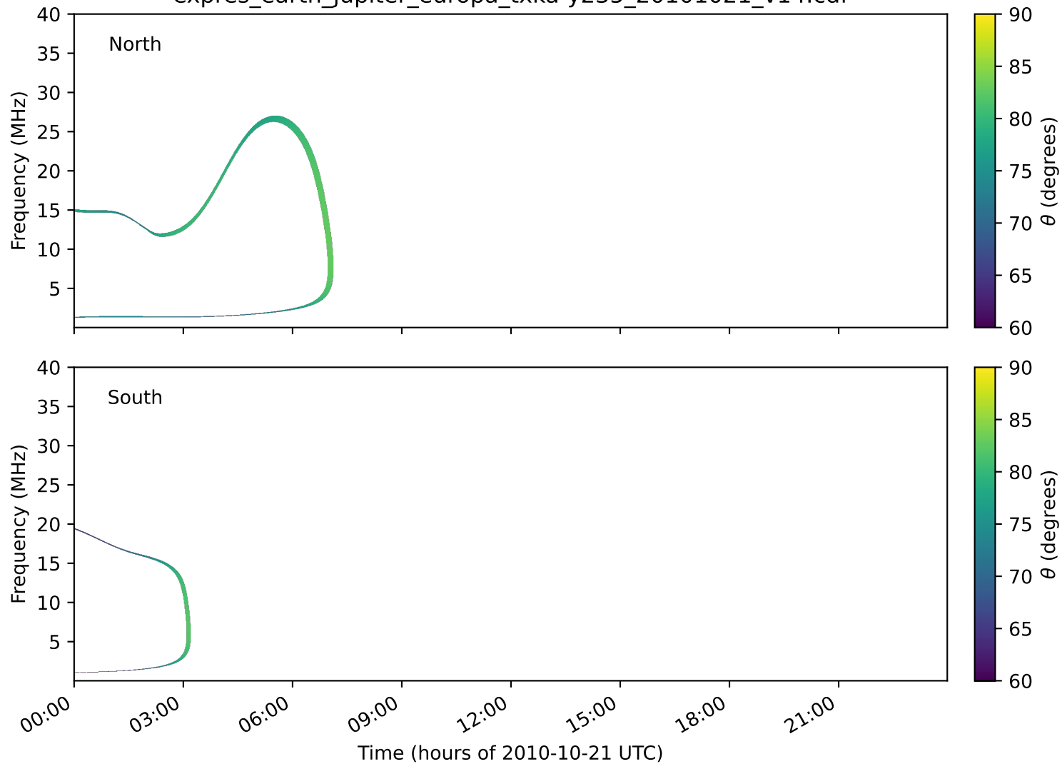
expres_earth_jupiter_europa_txka-y235_20101021_v14.cdf
