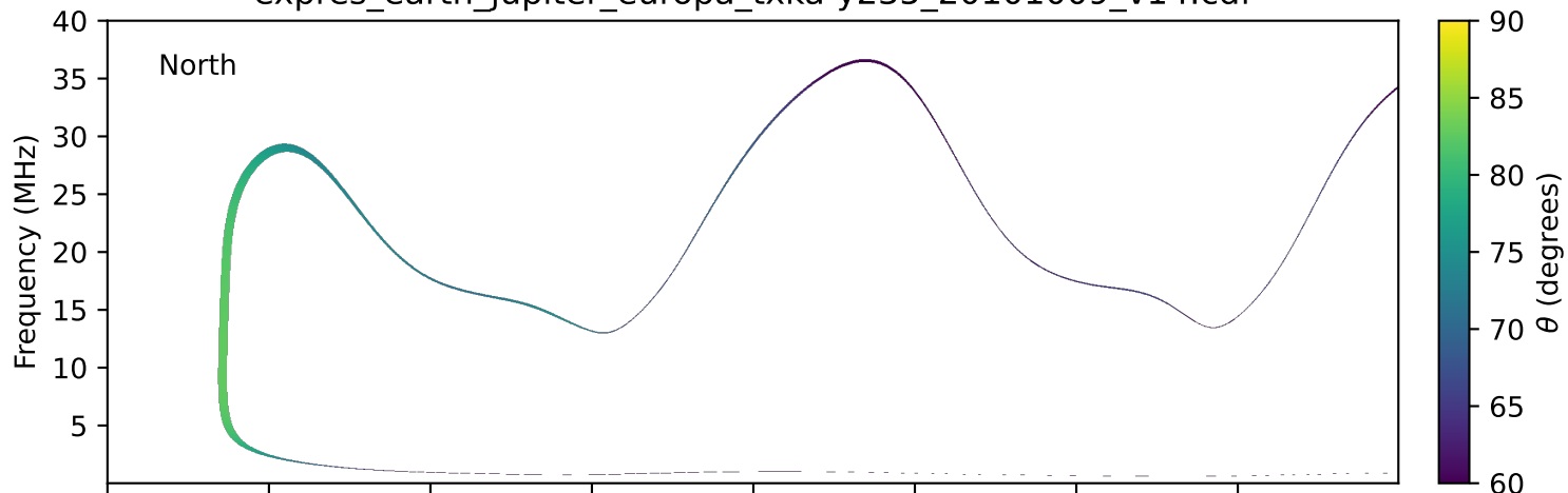
expres_earth_jupiter_europa_txka-y235_20101009_v14.cdf
