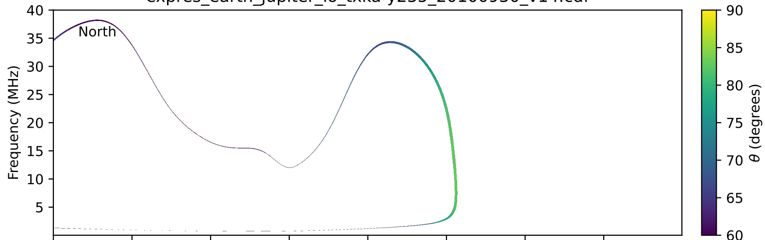
expres_earth_jupiter_io_txka-y235_20100930_v14.cdf
