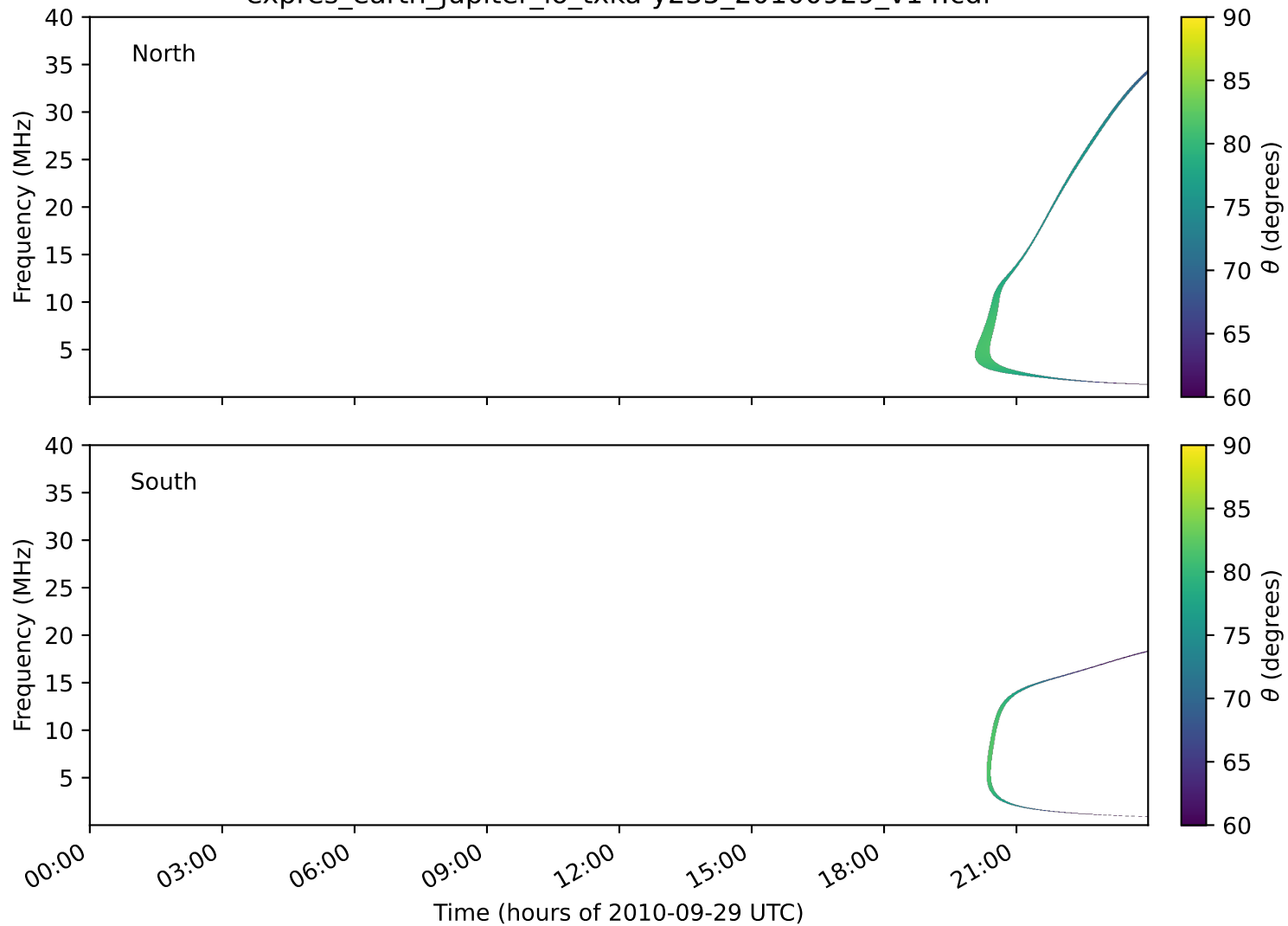
expres_earth_jupiter_io_txka-y235_20100929_v14.cdf
