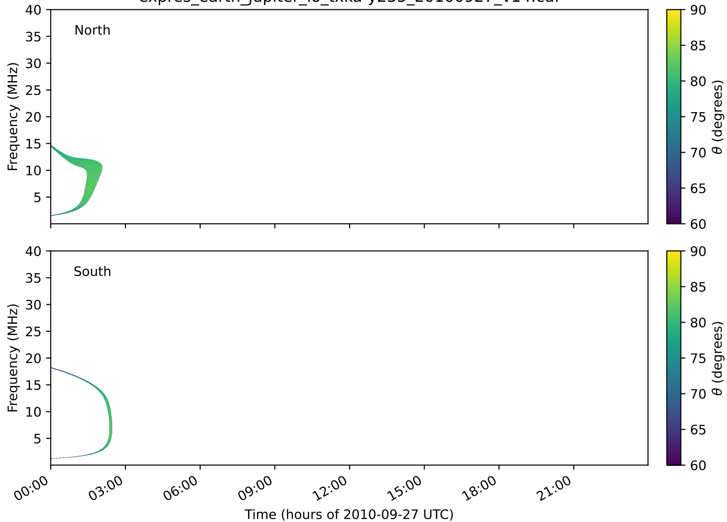
expres_earth_jupiter_io_txka-y235_20100927_v14.cdf
