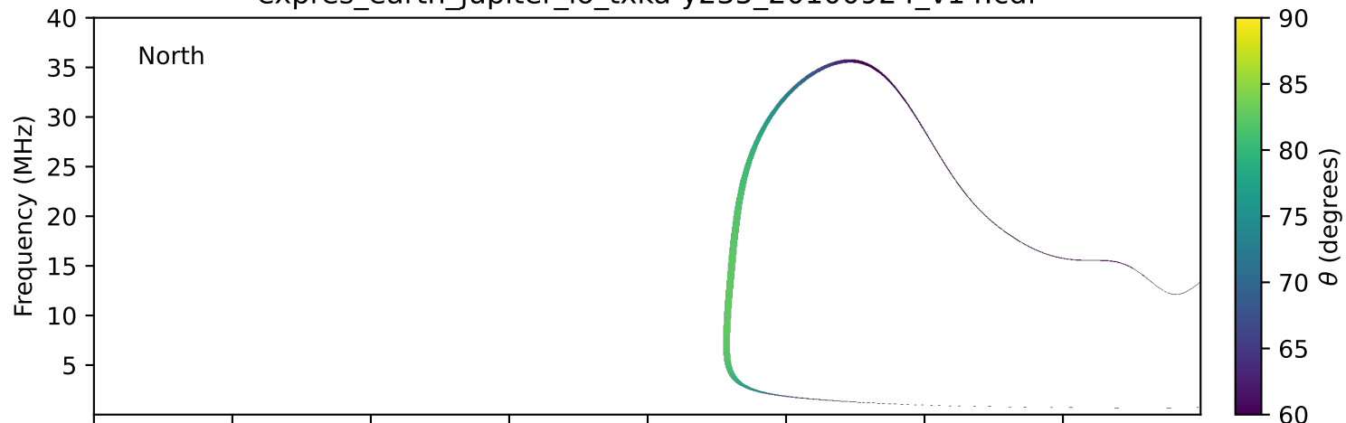
expres_earth_jupiter_io_txka-y235_20100924_v14.cdf
