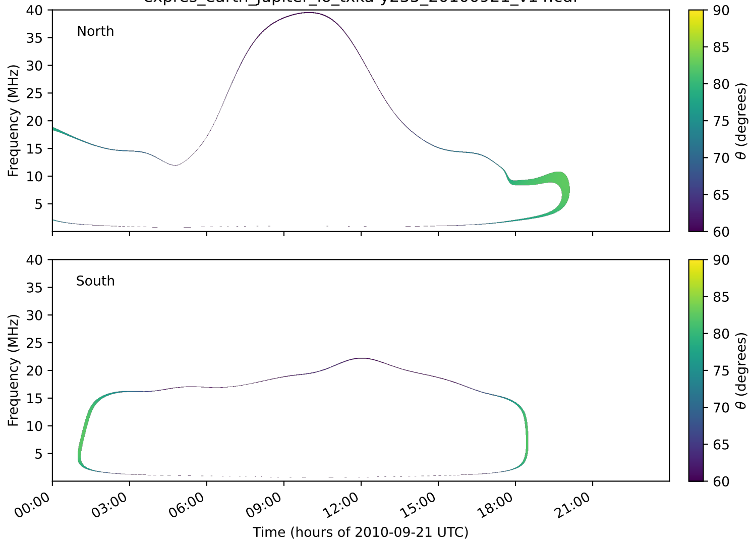
expres_earth_jupiter_io_txka-y235_20100921_v14.cdf
