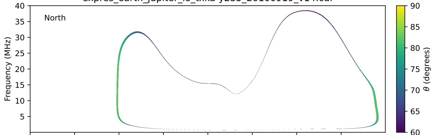
expres_earth_jupiter_io_txka-y235_20100919_v14.cdf
