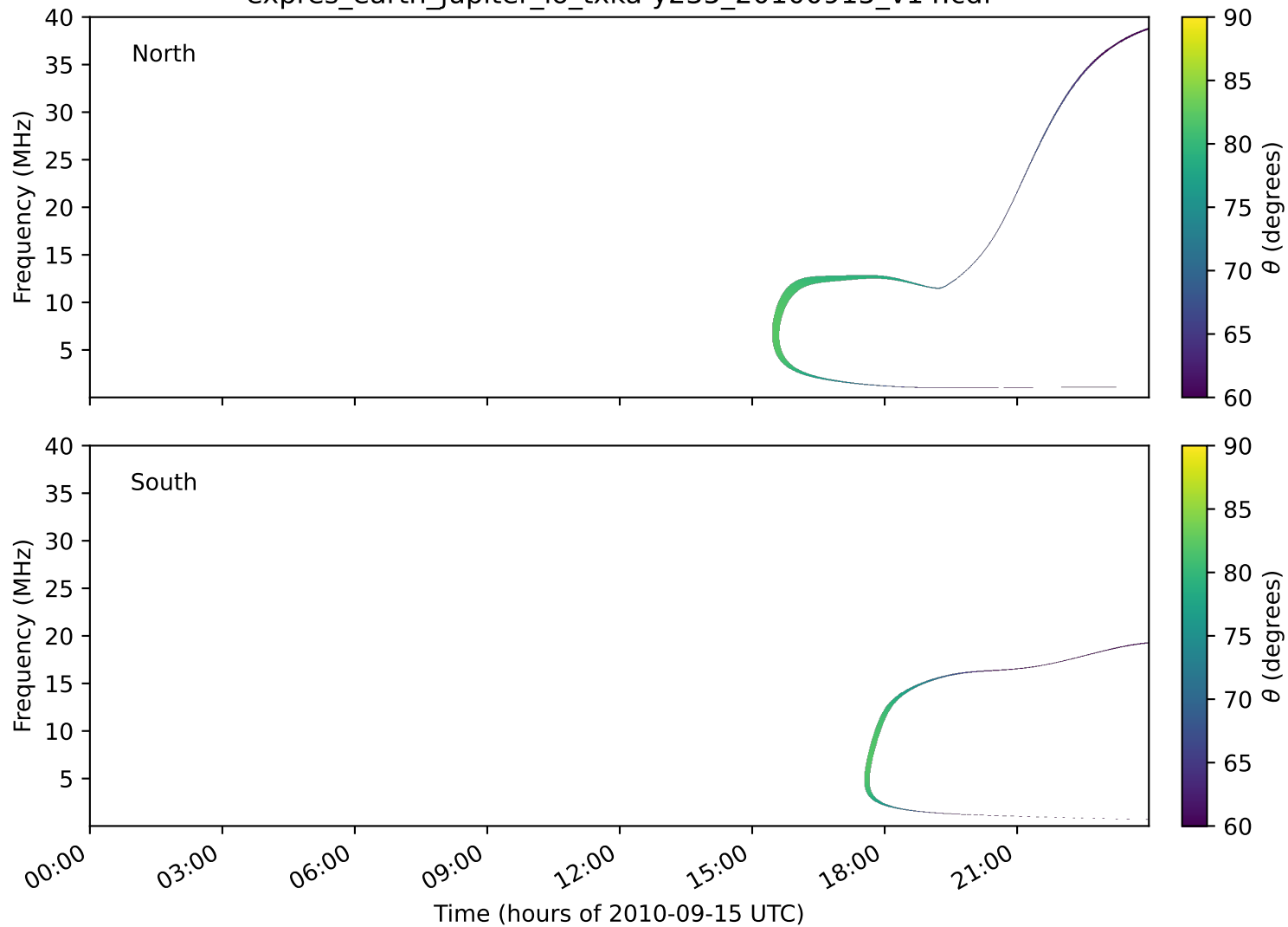
expres_earth_jupiter_io_txka-y235_20100915_v14.cdf
