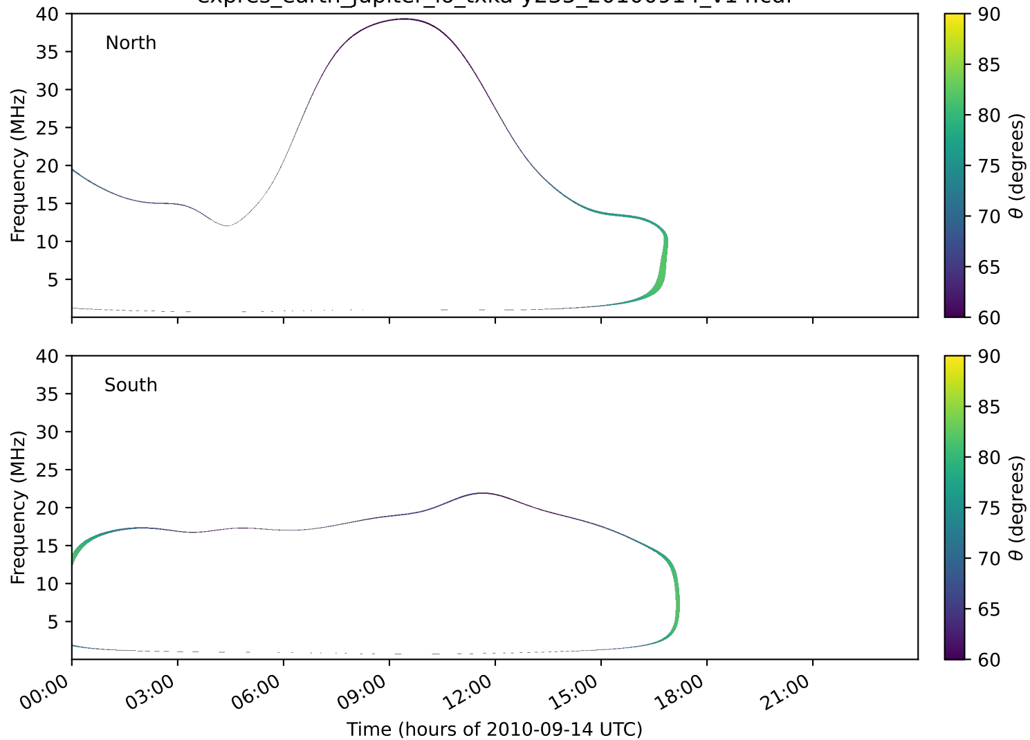
expres_earth_jupiter_io_txka-y235_20100914_v14.cdf
