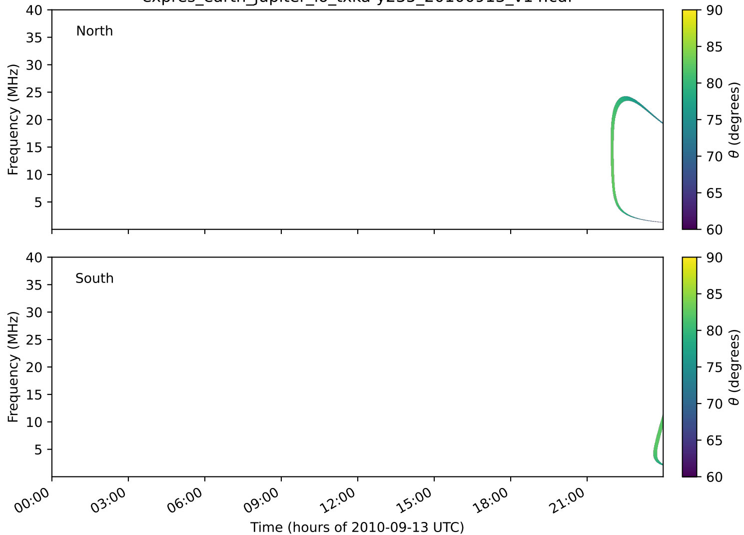
expres_earth_jupiter_io_txka-y235_20100913_v14.cdf
