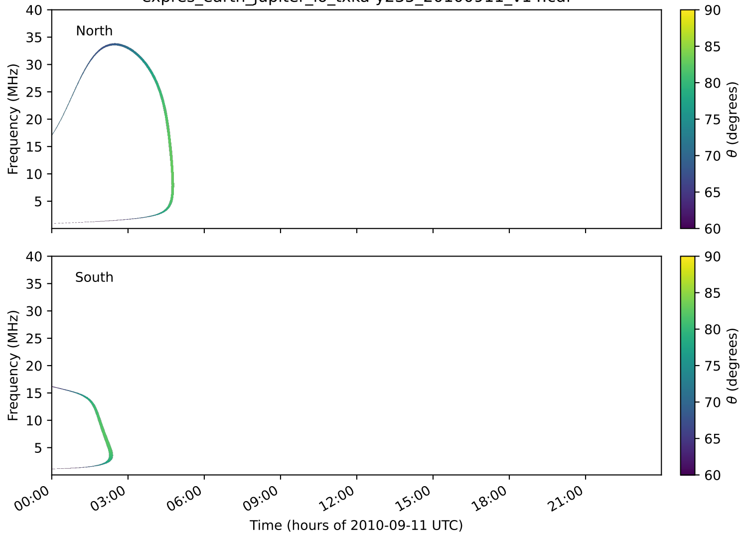
expres_earth_jupiter_io_txka-y235_20100911_v14.cdf
