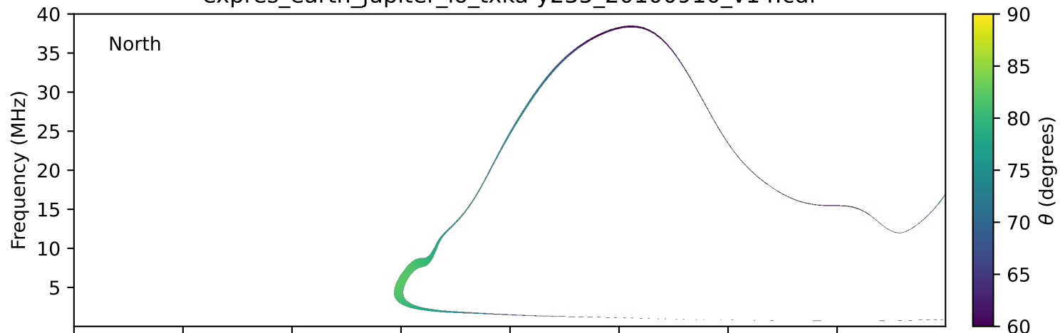
expres_earth_jupiter_io_txka-y235_20100910_v14.cdf
