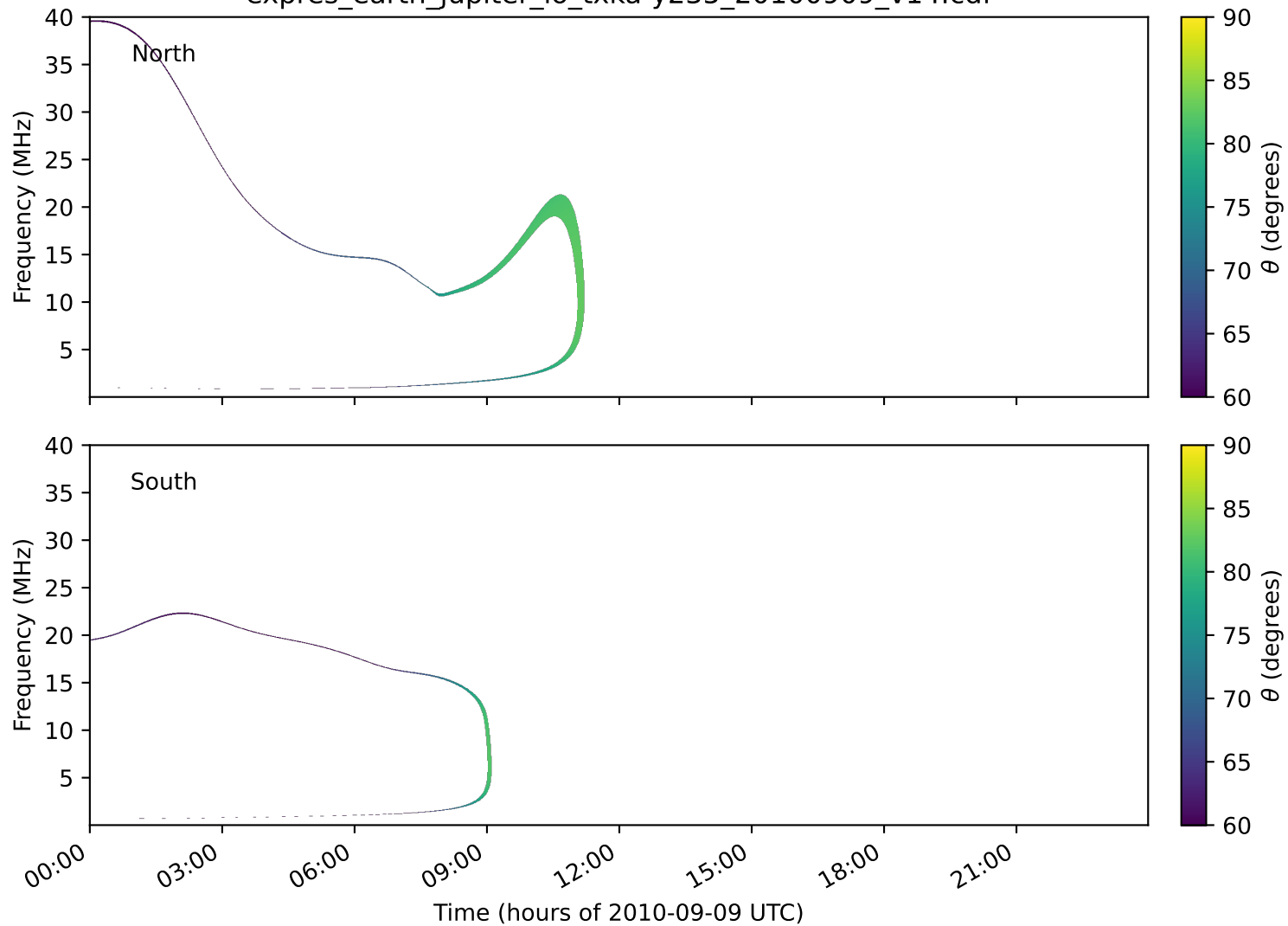
expres_earth_jupiter_io_txka-y235_20100909_v14.cdf
