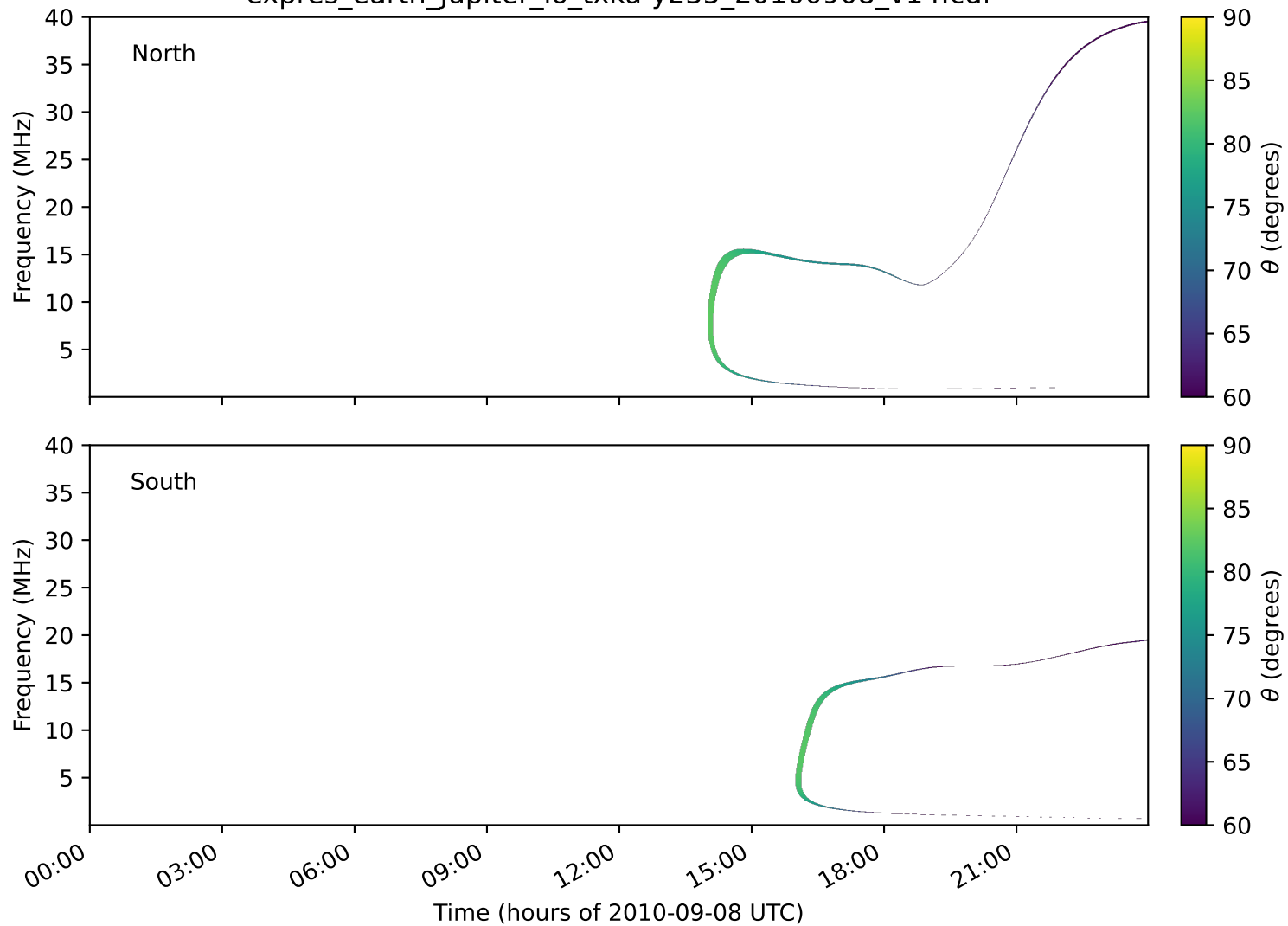
expres_earth_jupiter_io_txka-y235_20100908_v14.cdf
