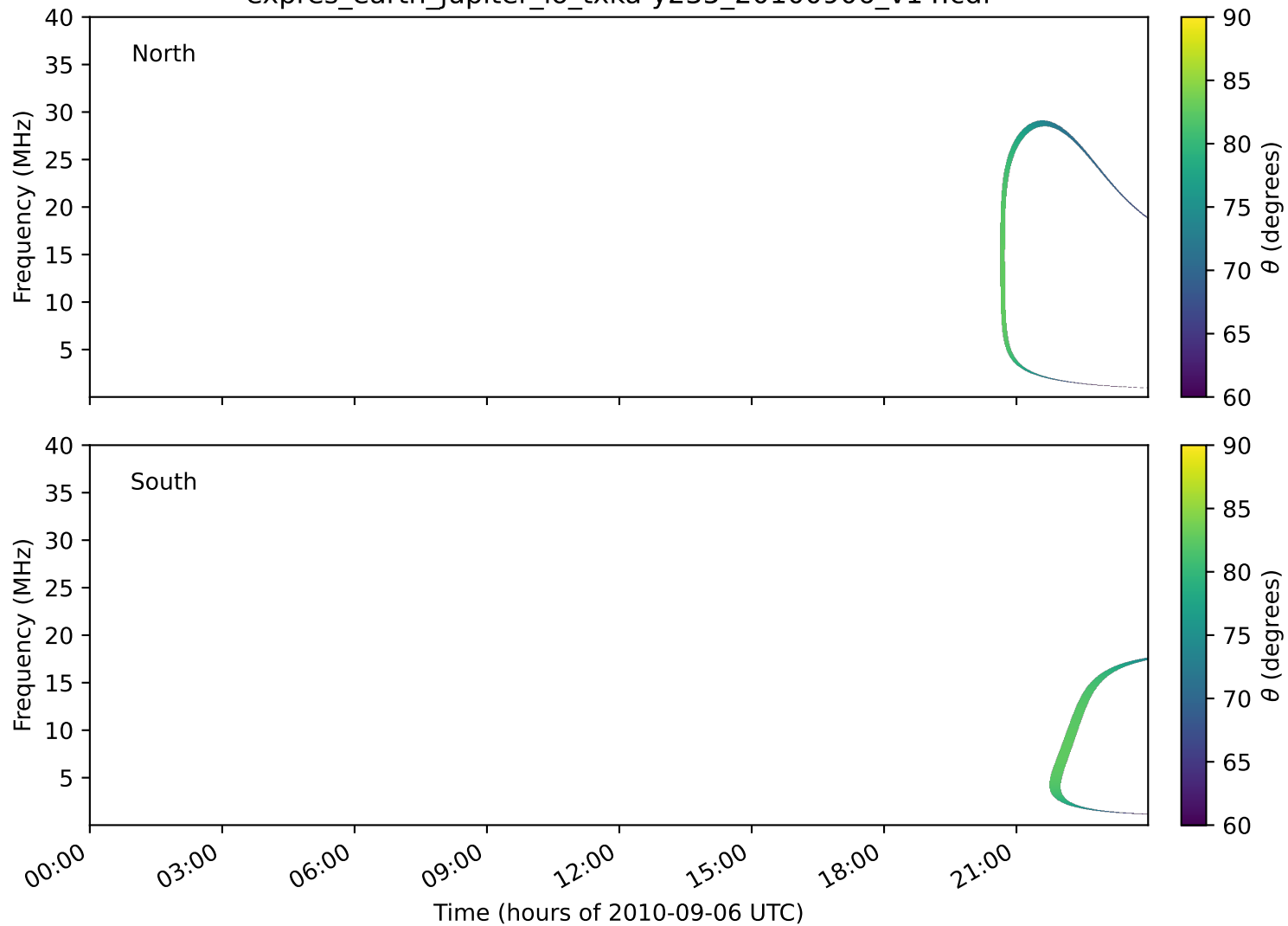
expres_earth_jupiter_io_txka-y235_20100906_v14.cdf
