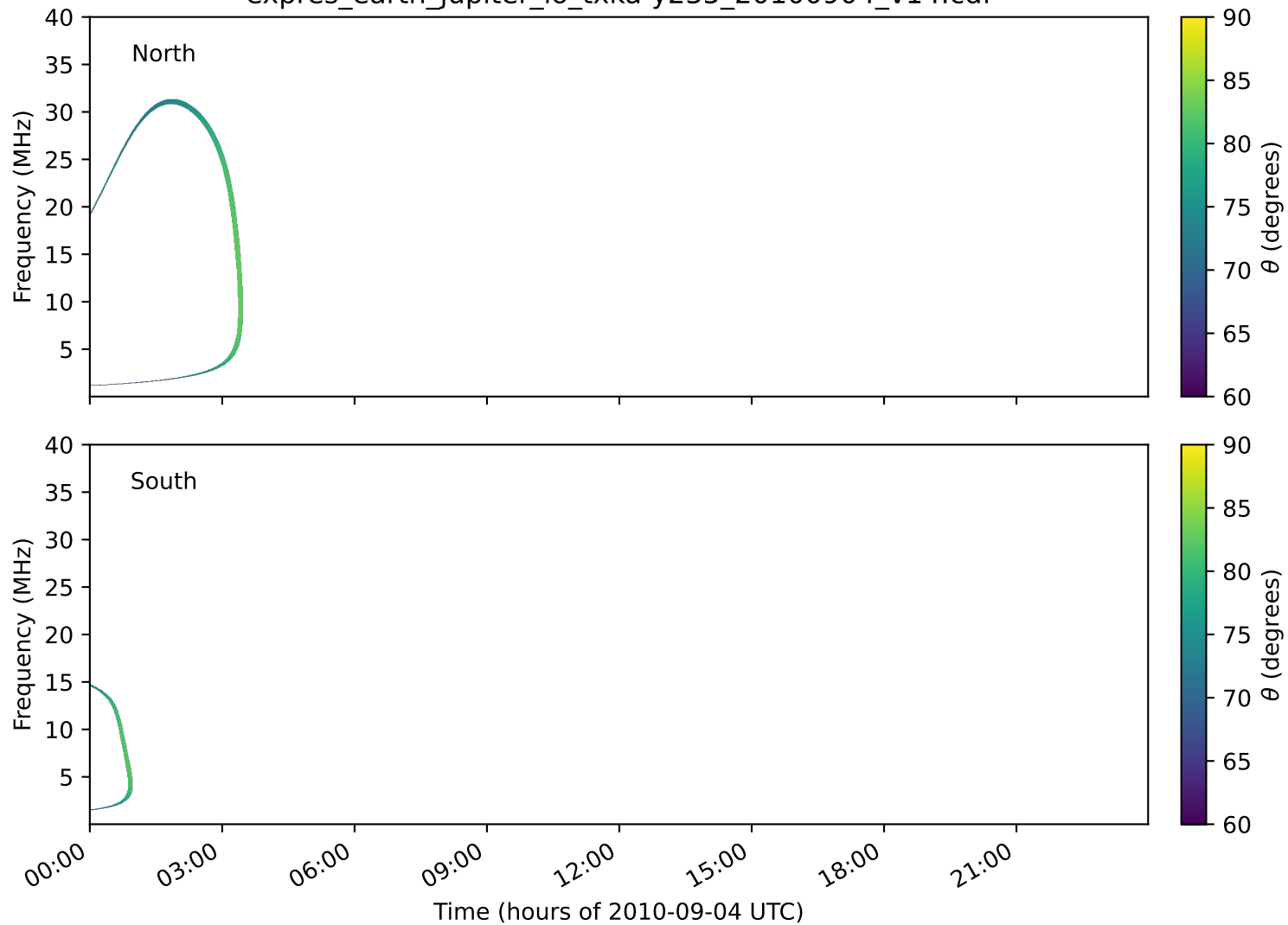
expres_earth_jupiter_io_txka-y235_20100904_v14.cdf
