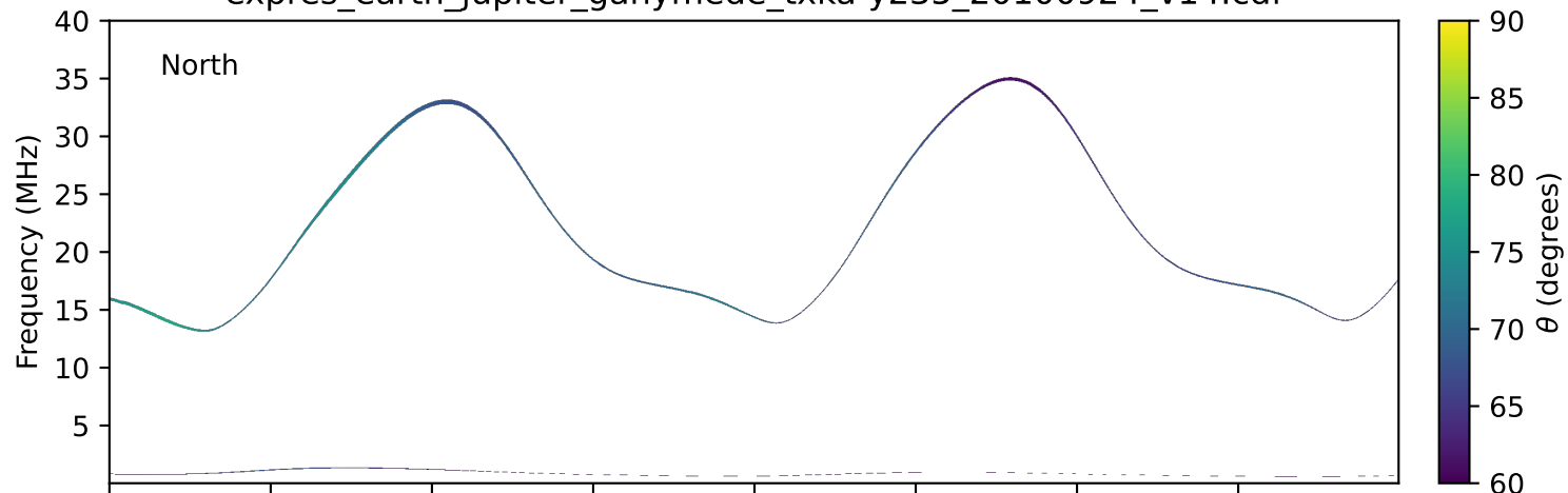
expres_earth_jupiter_ganymede_txka-y235_20100924_v14.cdf
