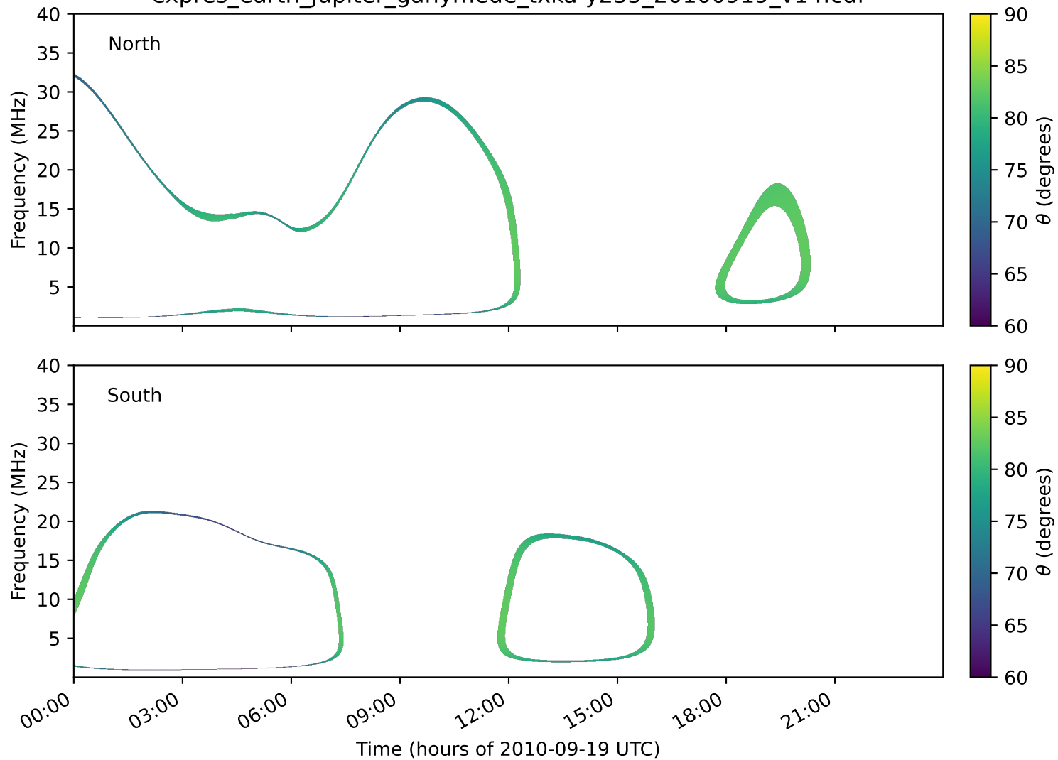
expres_earth_jupiter_ganymede_txka-y235_20100919_v14.cdf
