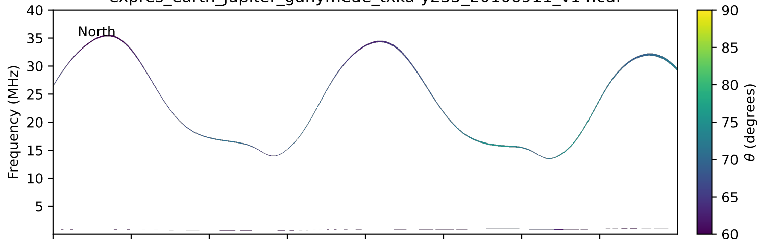
expres_earth_jupiter_ganymede_txka-y235_20100911_v14.cdf
