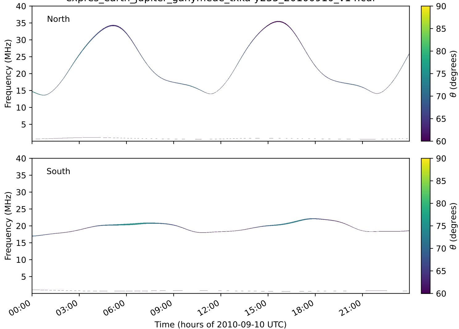
expres_earth_jupiter_ganymede_txka-y235_20100910_v14.cdf
