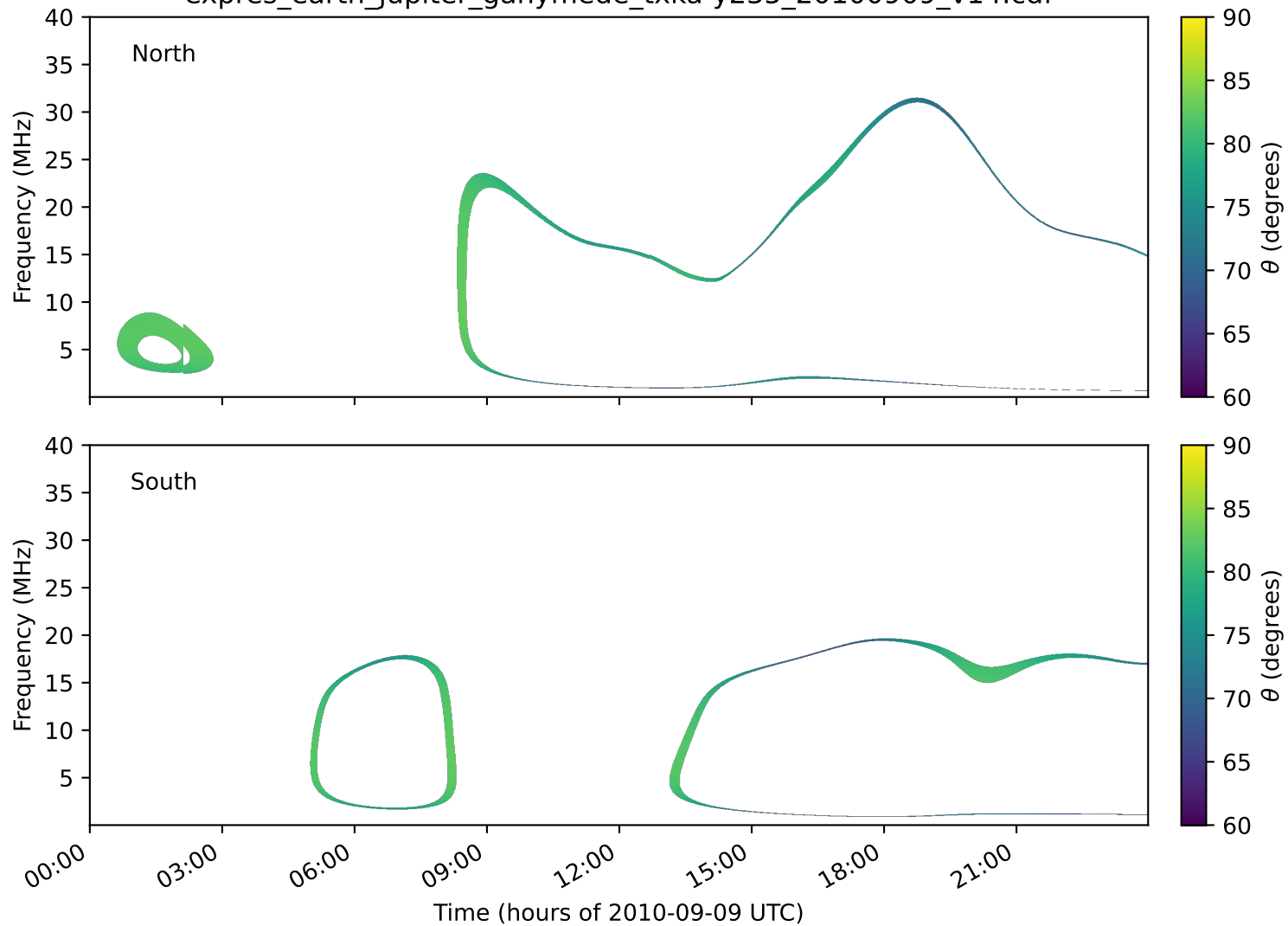
expres_earth_jupiter_ganymede_txka-y235_20100909_v14.cdf
