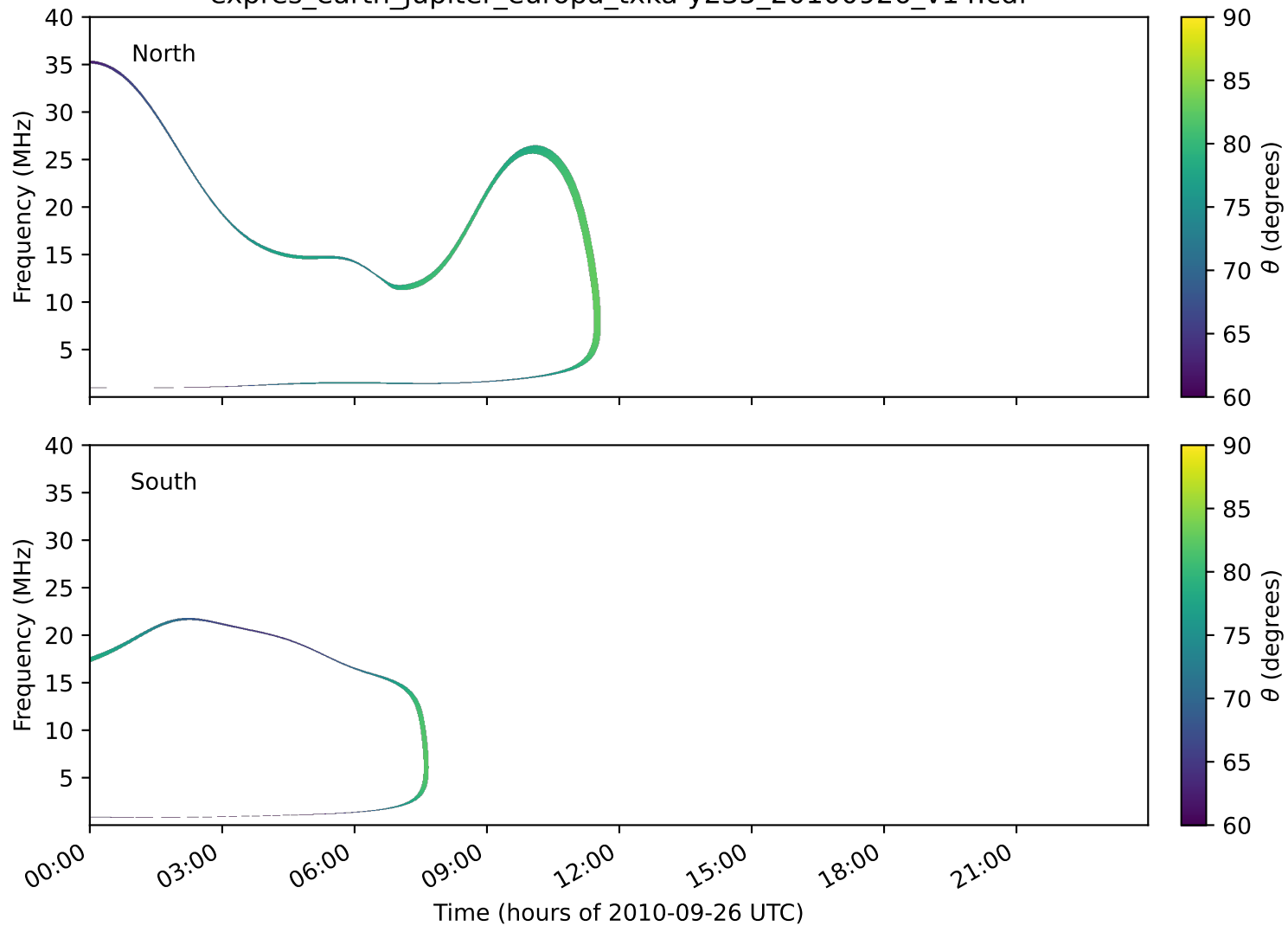
expres_earth_jupiter_europa_txka-y235_20100926_v14.cdf
