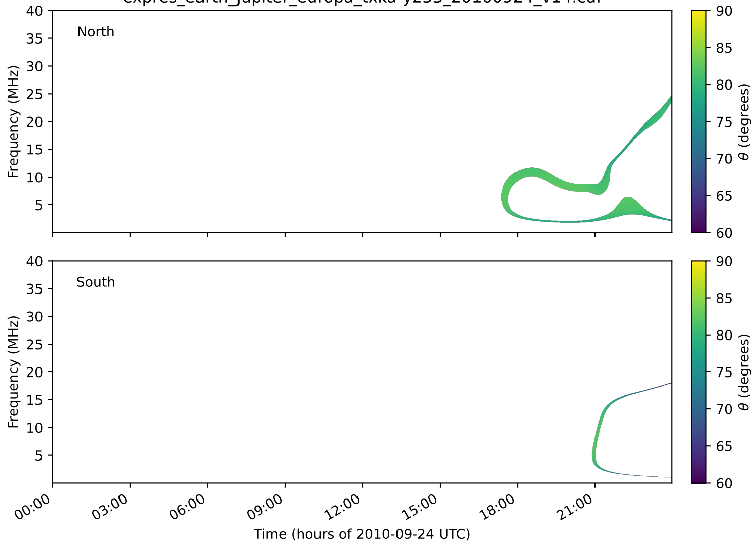
expres_earth_jupiter_europa_txka-y235_20100924_v14.cdf
