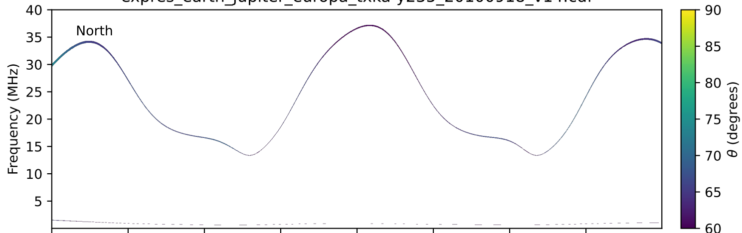
expres_earth_jupiter_europa_txka-y235_20100918_v14.cdf
