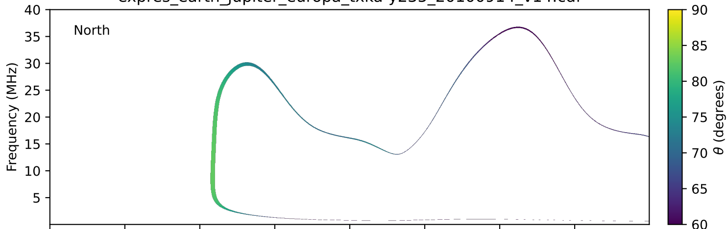
expres_earth_jupiter_europa_txka-y235_20100914_v14.cdf
