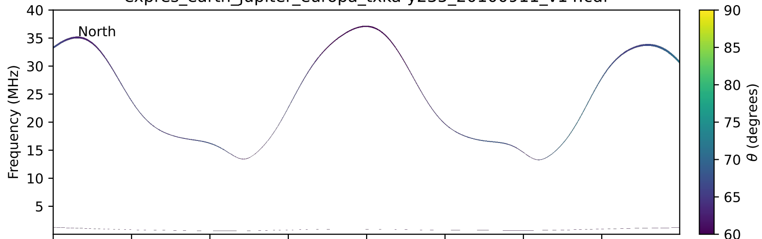
expres_earth_jupiter_europa_txka-y235_20100911_v14.cdf
