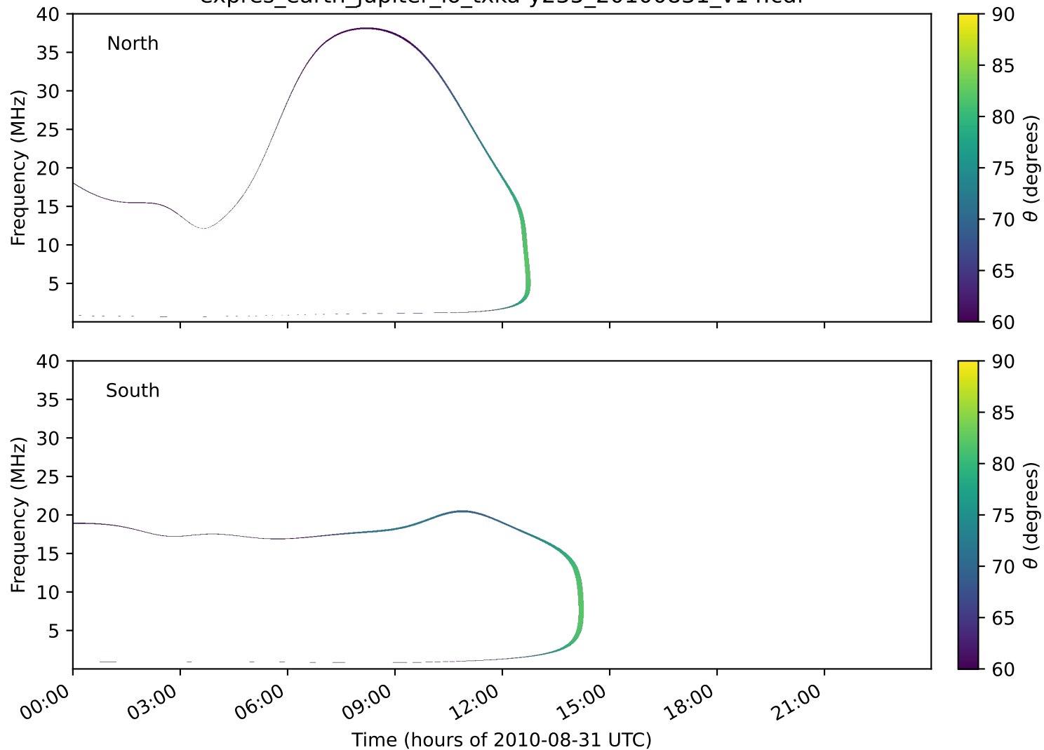
expres_earth_jupiter_io_txka-y235_20100831_v14.cdf
