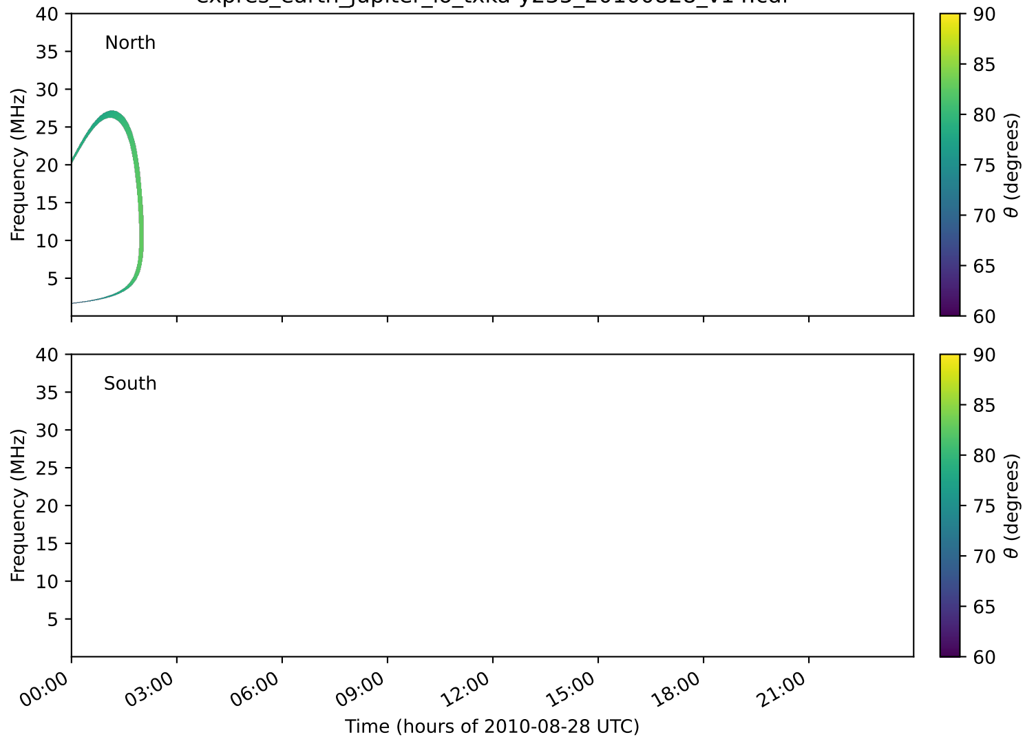
expres_earth_jupiter_io_txka-y235_20100828_v14.cdf
