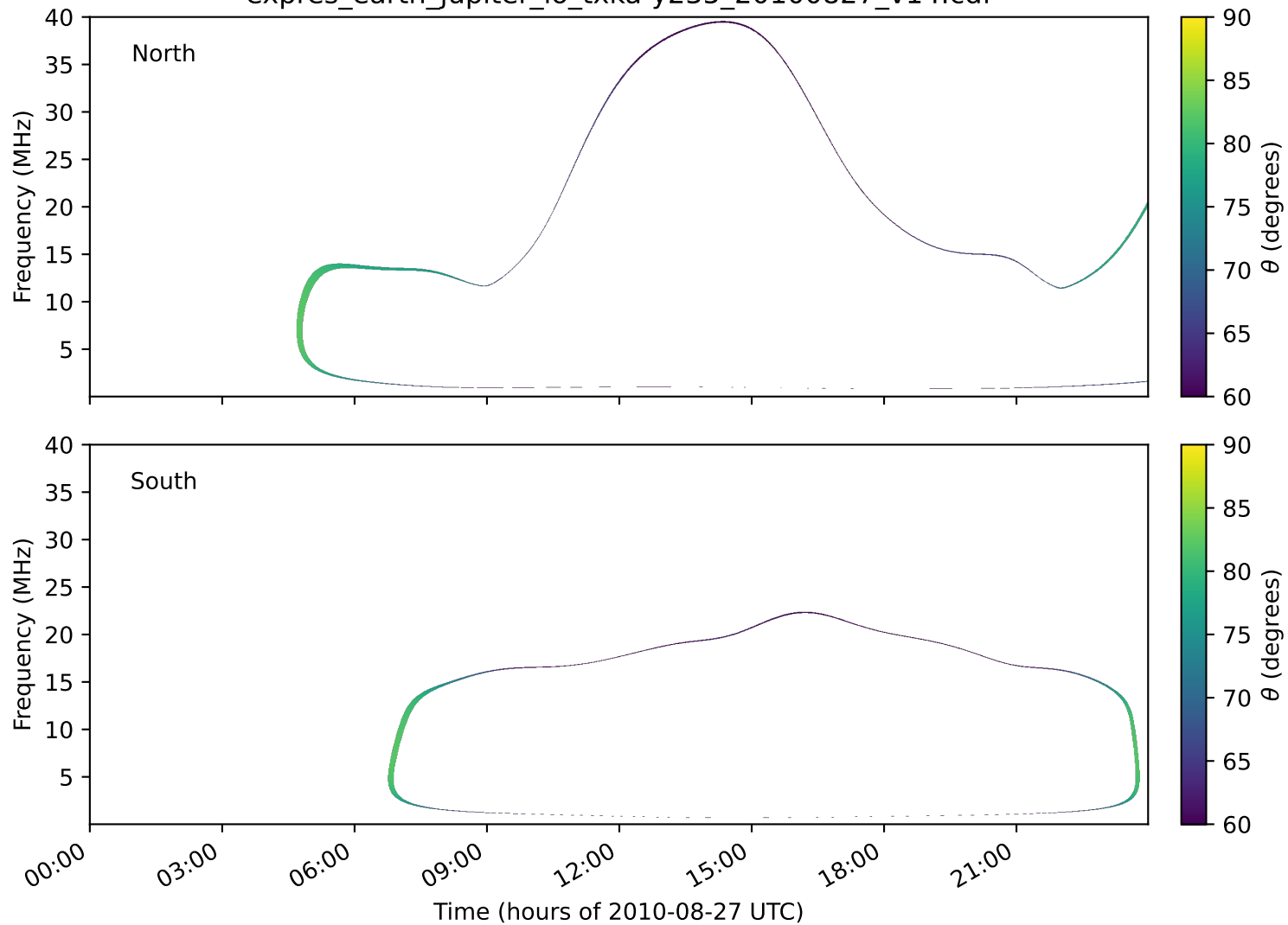
expres_earth_jupiter_io_txka-y235_20100827_v14.cdf
