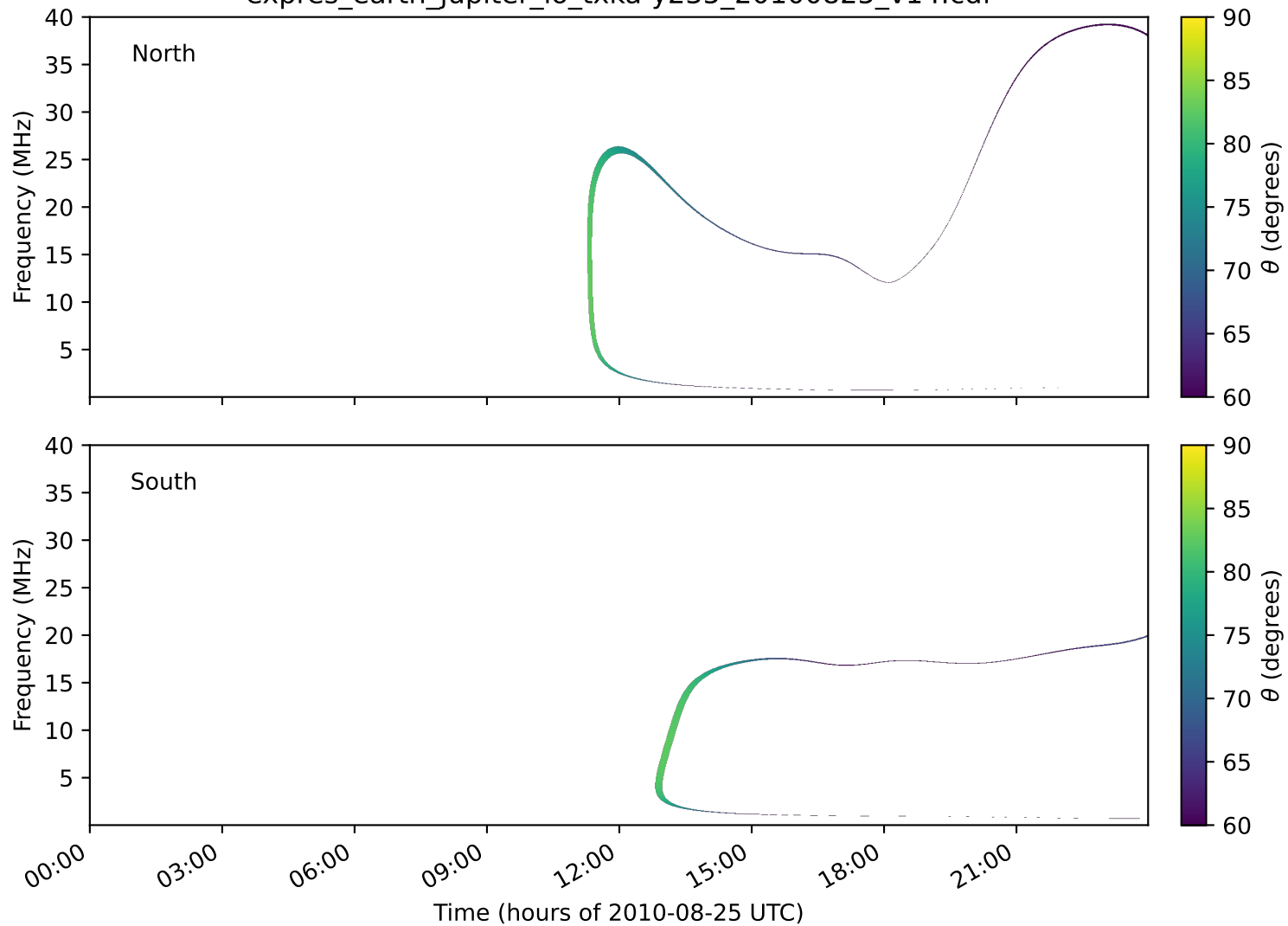
expres_earth_jupiter_io_txka-y235_20100825_v14.cdf
