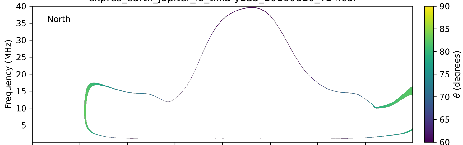
expres_earth_jupiter_io_txka-y235_20100820_v14.cdf
