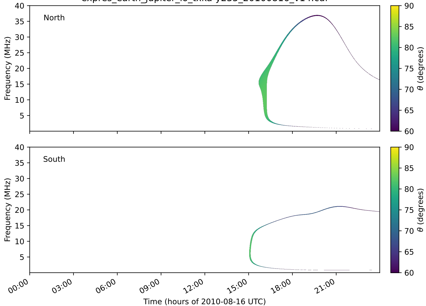
expres_earth_jupiter_io_txka-y235_20100816_v14.cdf
