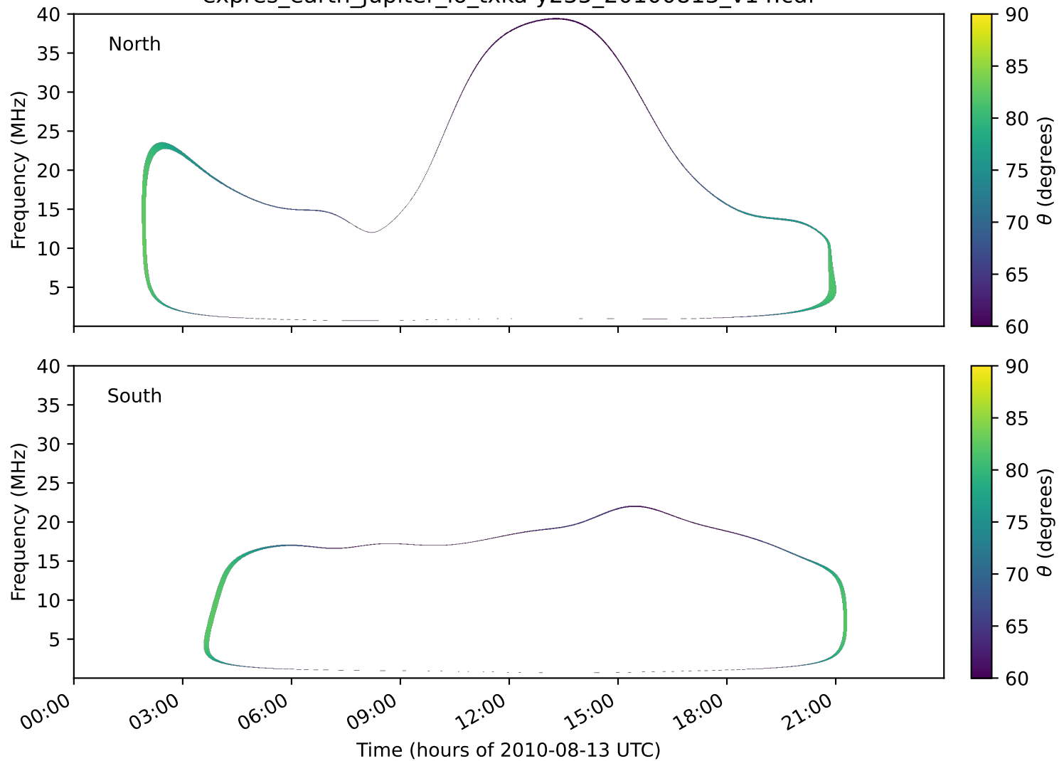
expres_earth_jupiter_io_txka-y235_20100813_v14.cdf
