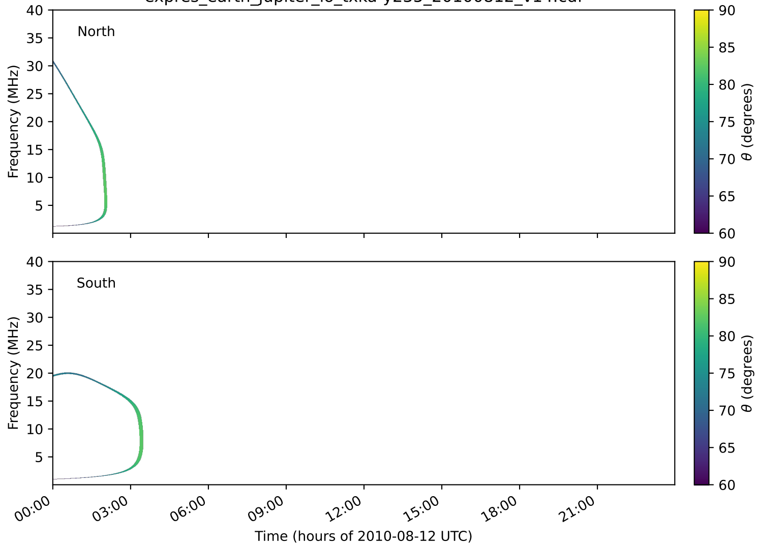
expres_earth_jupiter_io_txka-y235_20100812_v14.cdf
