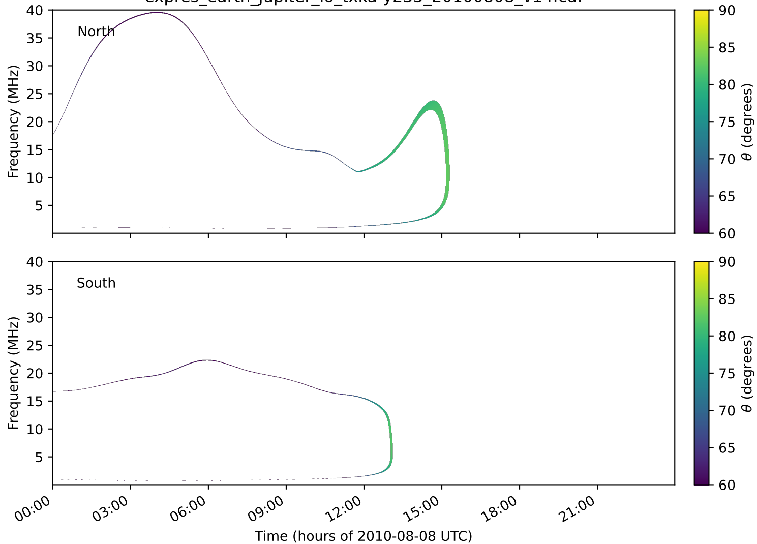
expres_earth_jupiter_io_txka-y235_20100808_v14.cdf
