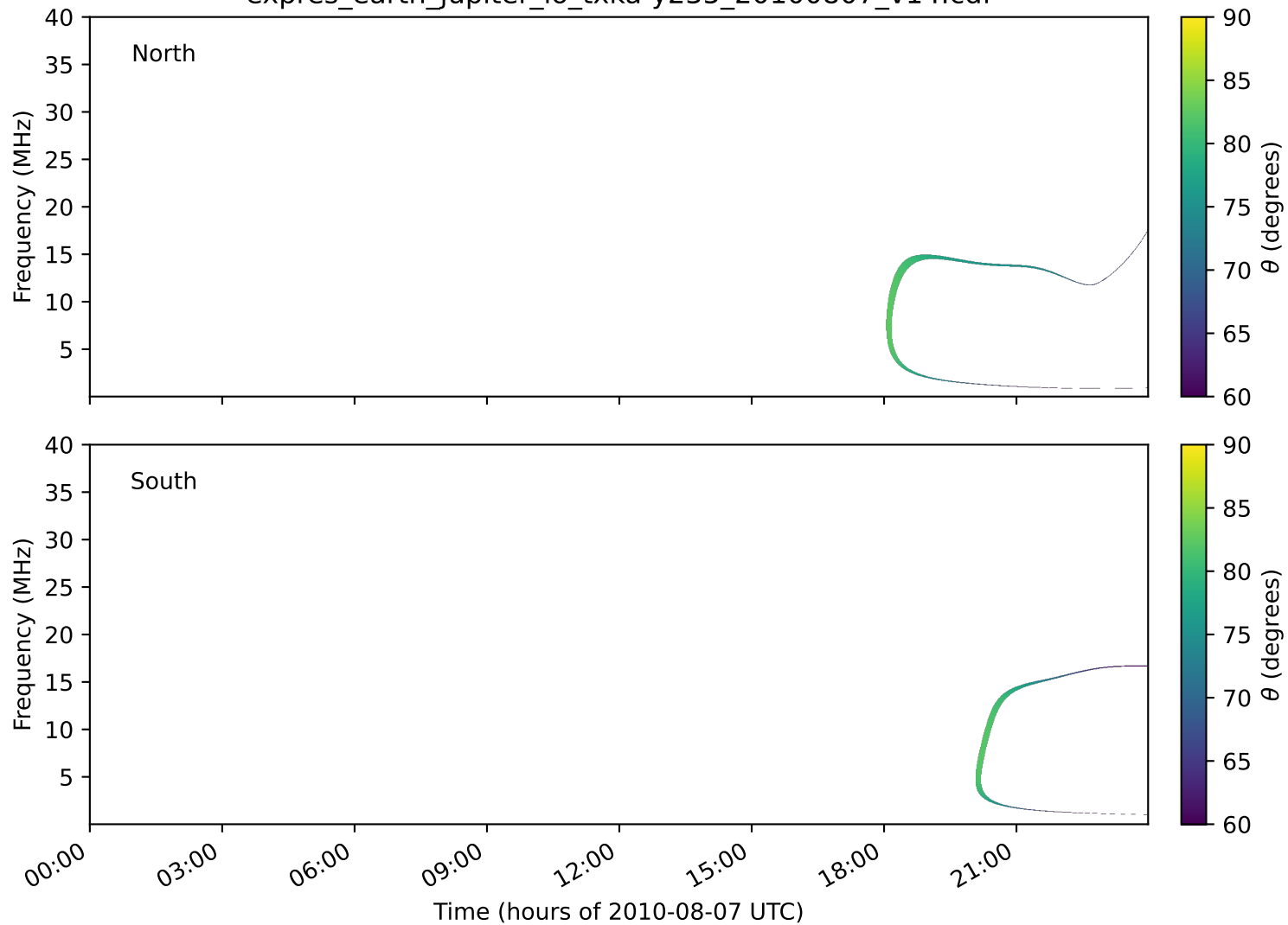
expres_earth_jupiter_io_txka-y235_20100807_v14.cdf
