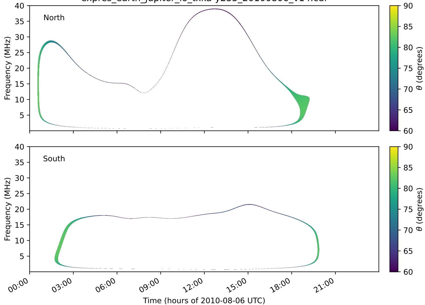
expres_earth_jupiter_io_txka-y235_20100806_v14.cdf
