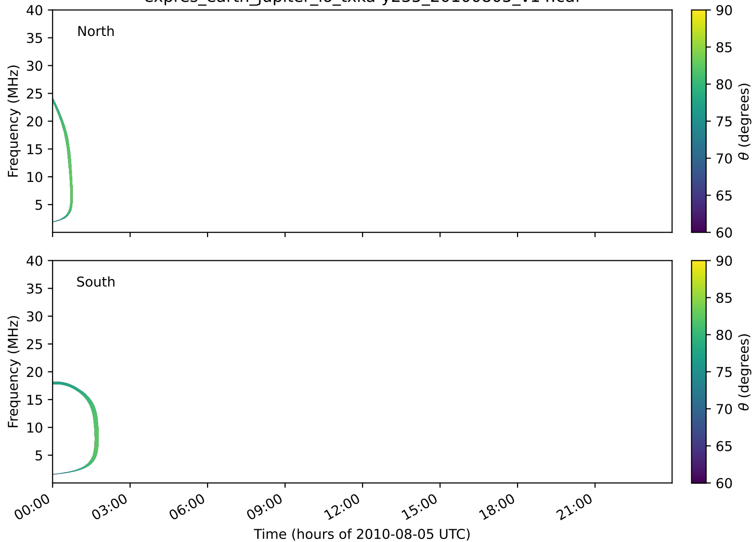
expres_earth_jupiter_io_txka-y235_20100805_v14.cdf
