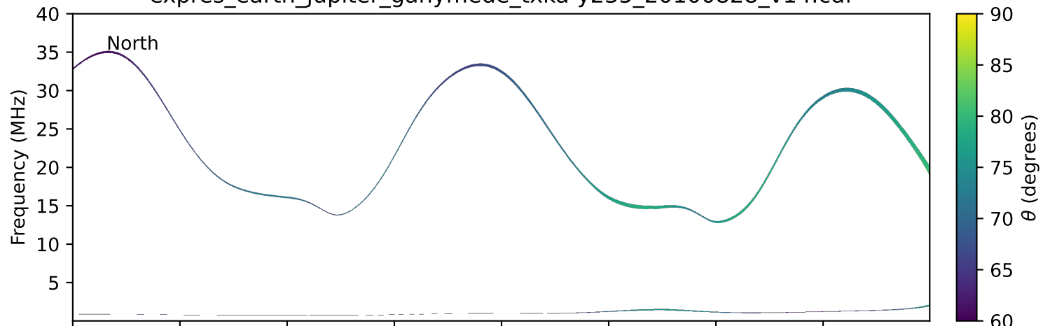
expres_earth_jupiter_ganymede_txka-y235_20100828_v14.cdf
