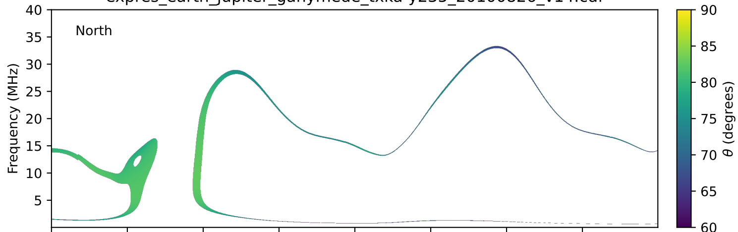
expres_earth_jupiter_ganymede_txka-y235_20100826_v14.cdf
