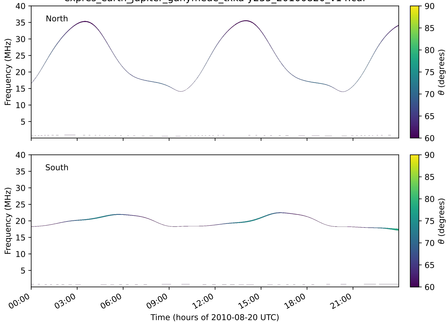
expres_earth_jupiter_ganymede_txka-y235_20100820_v14.cdf
