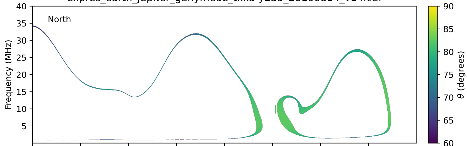
expres_earth_jupiter_ganymede_txka-y235_20100814_v14.cdf
