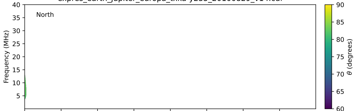
expres_earth_jupiter_europa_txka-y235_20100829_v14.cdf
