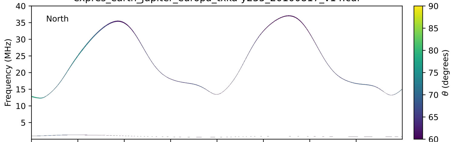
expres_earth_jupiter_europa_txka-y235_20100817_v14.cdf
